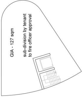
Cafe / Restaurant - Basement Plan
